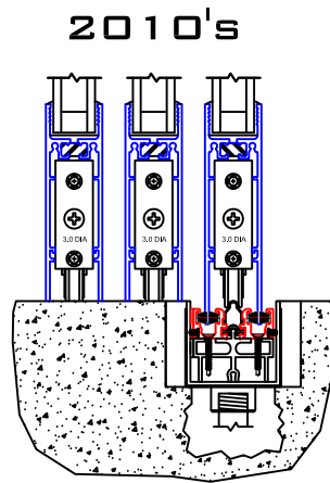
3070-T W/STAGGERED SUB-SILL
