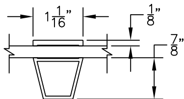
3 "STEEL LOOK" GRID
