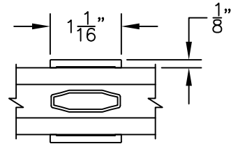
1A EXTRUDED SURFACE APPLIED GRID WITH EXTRUDED SHADOW BAR
