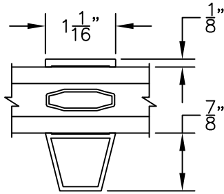
1 "STEEL LOOK" GRID WITH EXTRUDED SHADOW BAR
