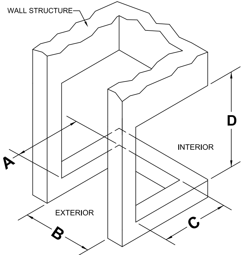
ISOMETRIC VIEW
