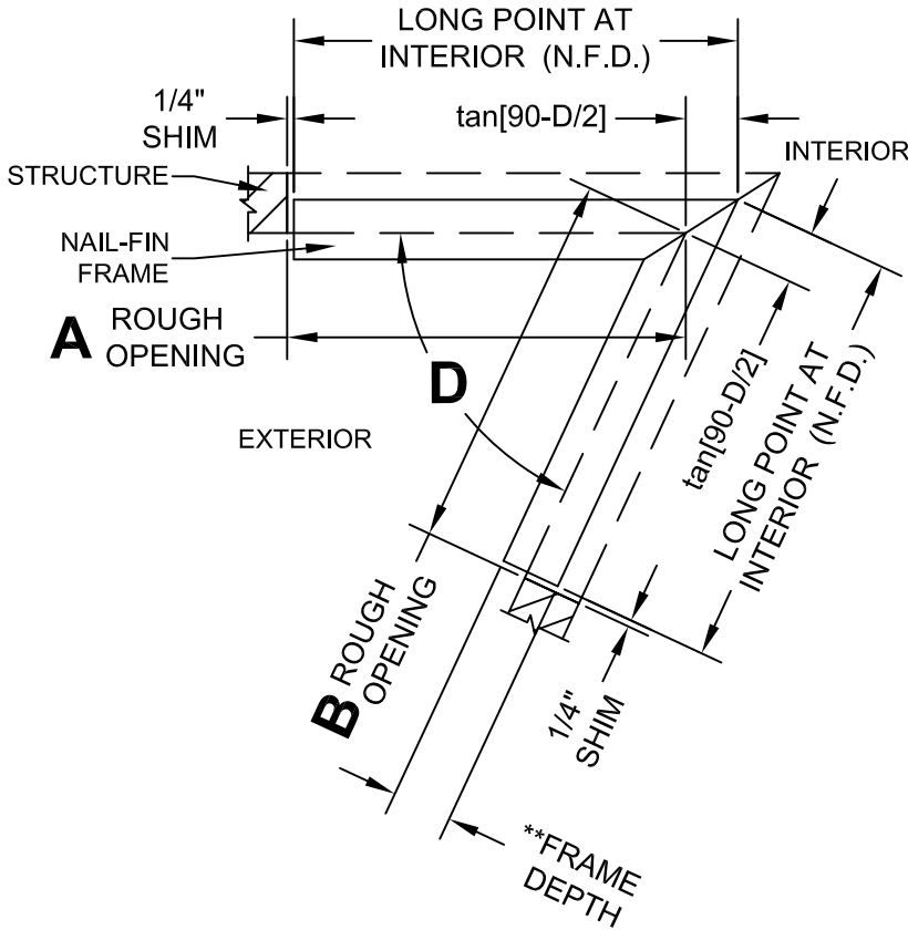
PLAN VIEW
